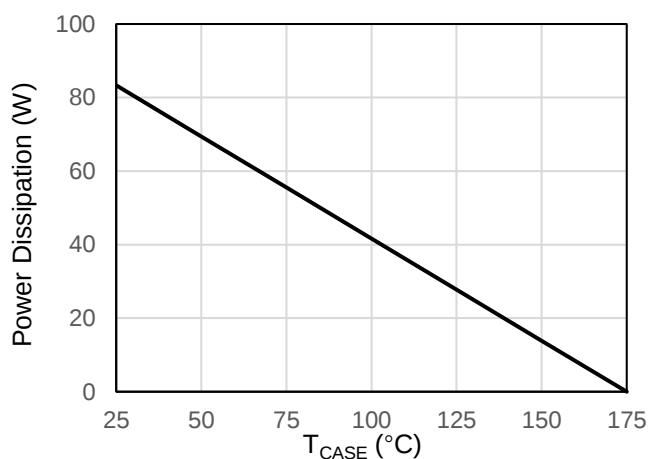
Figure 6: Power De-rating
