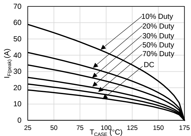
Figure 8: Current De-rating
