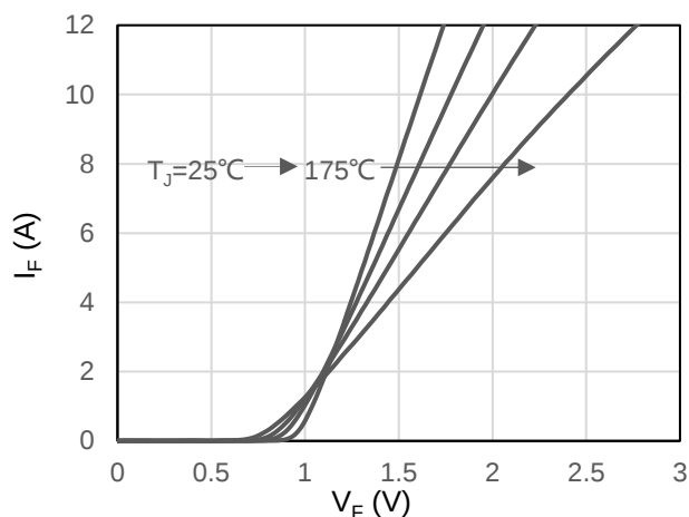
Figure 1: Forward Characteristics
