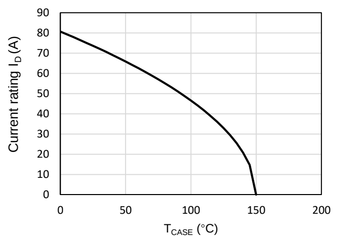
Figure 10: Current De-rating
