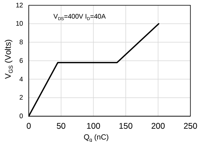
Figure 8: Gate-Charge Characteristics
