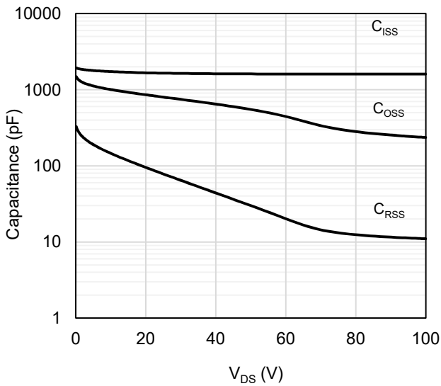
Figure 9: Capacitance Characteristics
