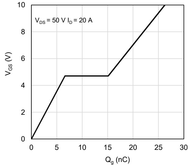
Figure 10: Gate-Charge Characteristics
