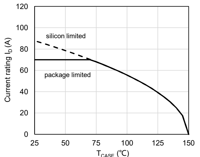
Figure 12: Current De-rating
