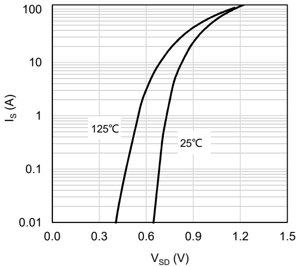
Figure 7: Body-Diode Characteristics
