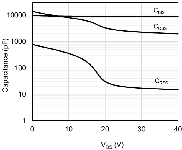
Figure 9: Capacitance Characteristics
