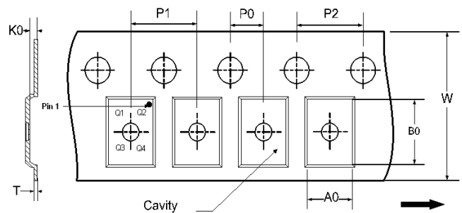
TAPE DIMENSIONS
