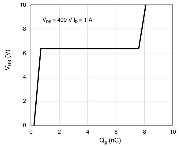
Figure 10: Gate-Charge Characteristics
