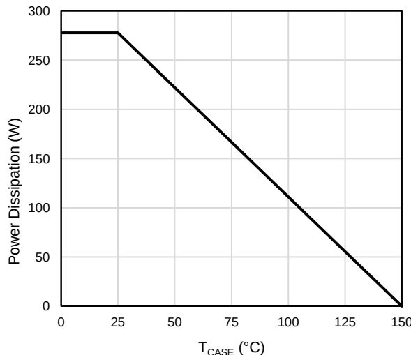
Figure 11: Power De-rating
