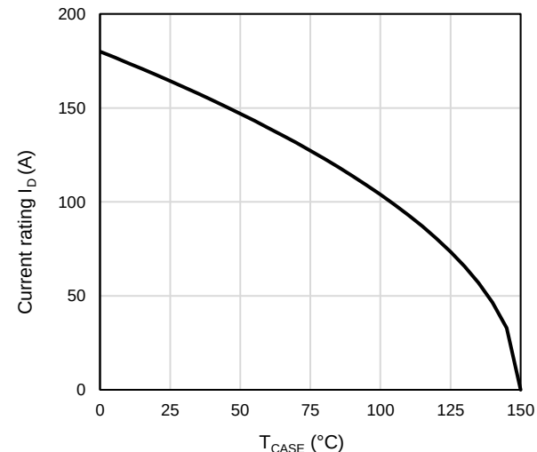
Figure 12: Current De-rating
