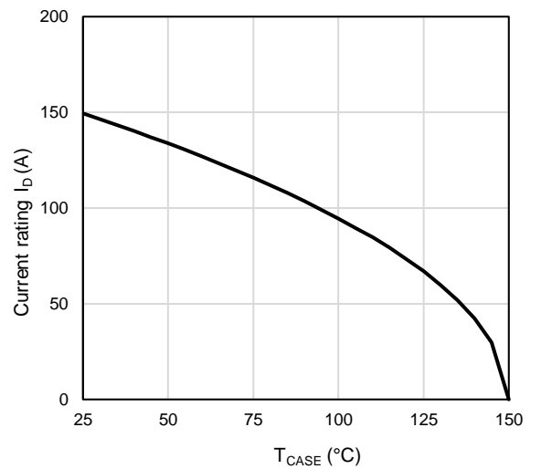
Figure 12: Current De-rating
