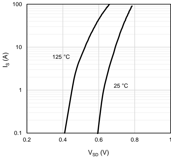
Figure 7: Body-Diode Characteristics
