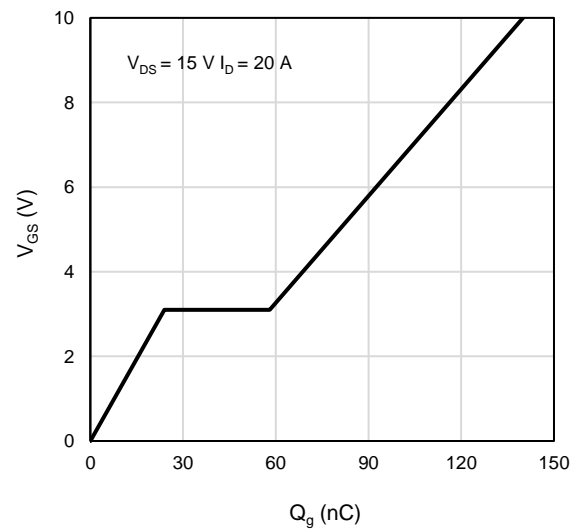
Figure 10: Gate-Charge Characteristics
